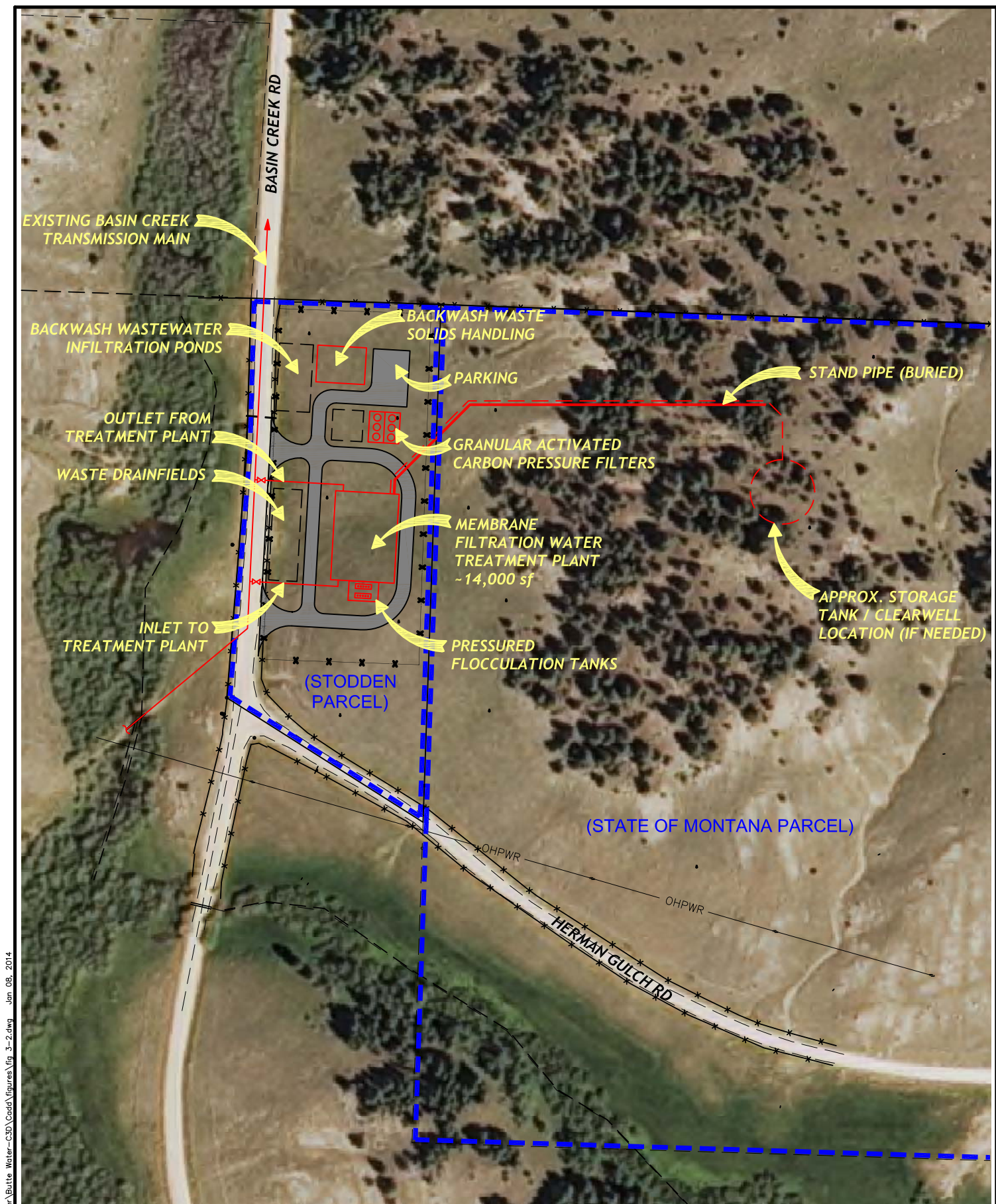
Butte - Silver Bow Water BASIN CREEK WATER TREATMENT PLANT Figure 3-2
